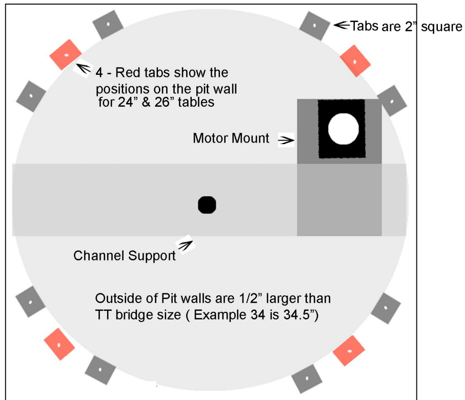
Overhead View of Turntable
