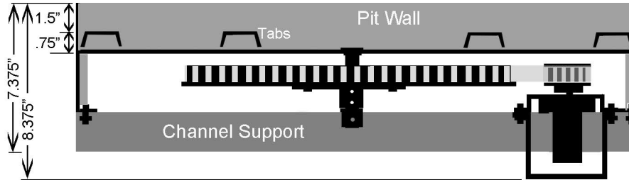
Side View of turntable
